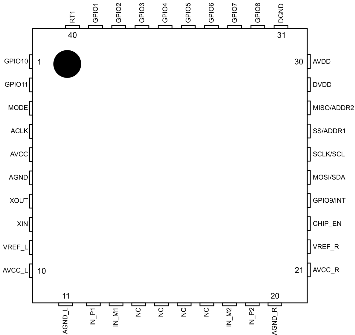
ES9822Q (Top View)
