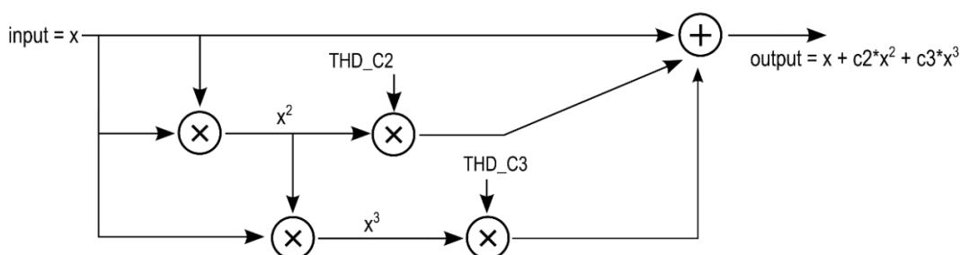
Figure 15 - TDM Compensation
