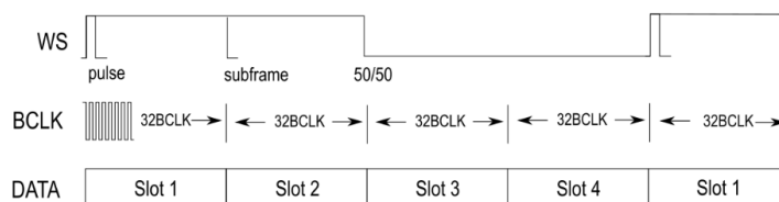
Figure 13 – TDM128 Mode
