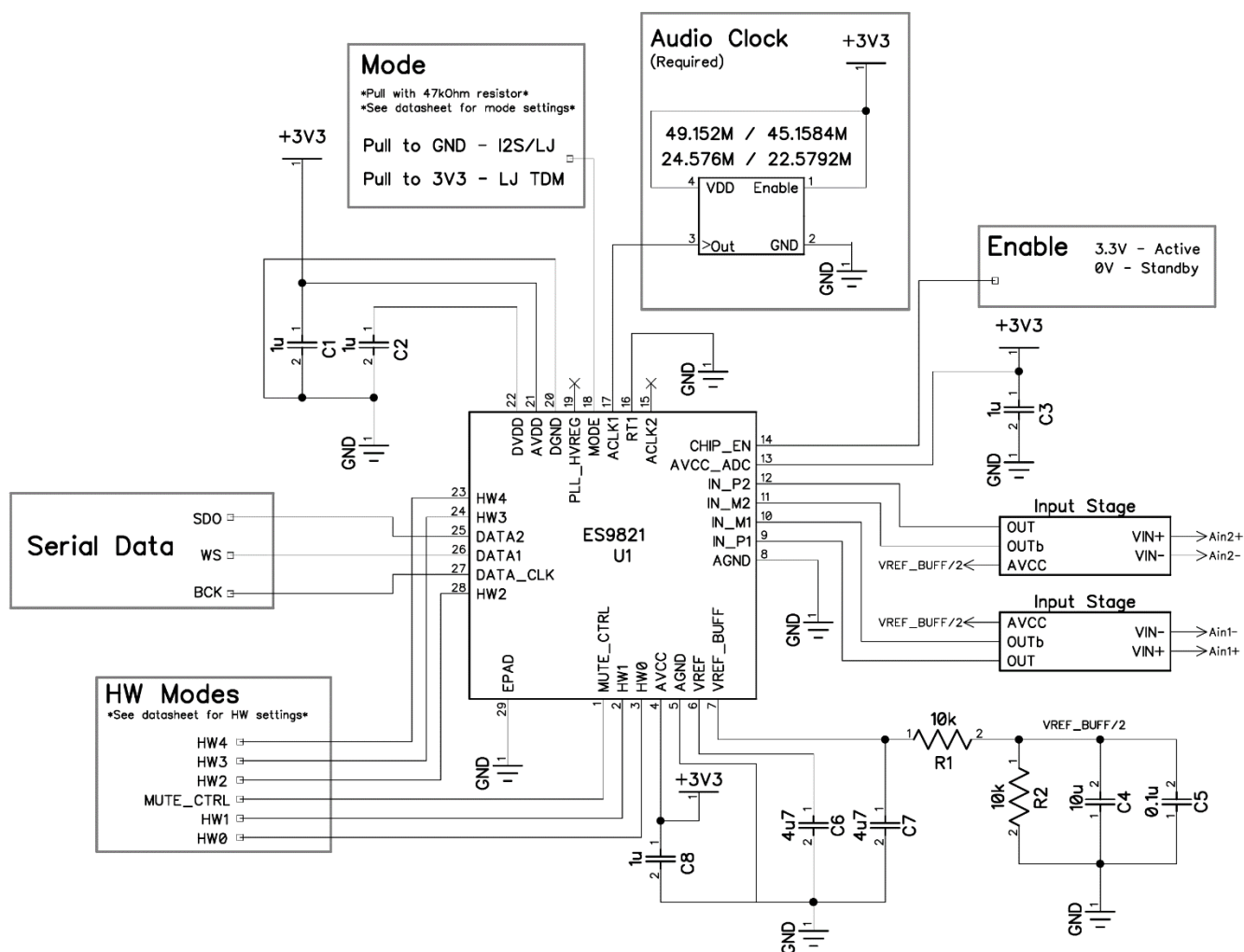
Figure 25 – ES9821Q Reference Schematic for Normal Operation in Hardware (HW) Mode
