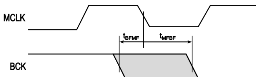
Figure 22 - 22/24MHz MCLK with BCK Phase Relationship
