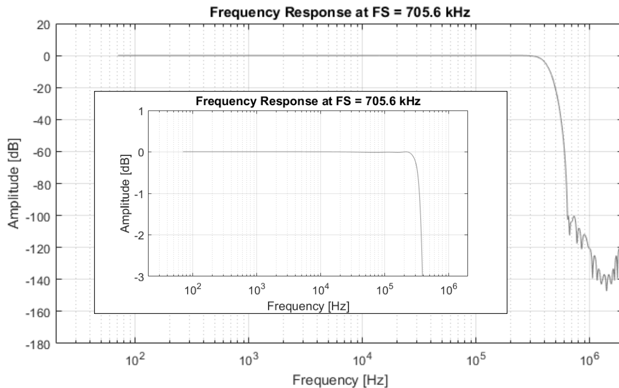
Figure 17 - Minimum Phase 64FS Frequency Response
