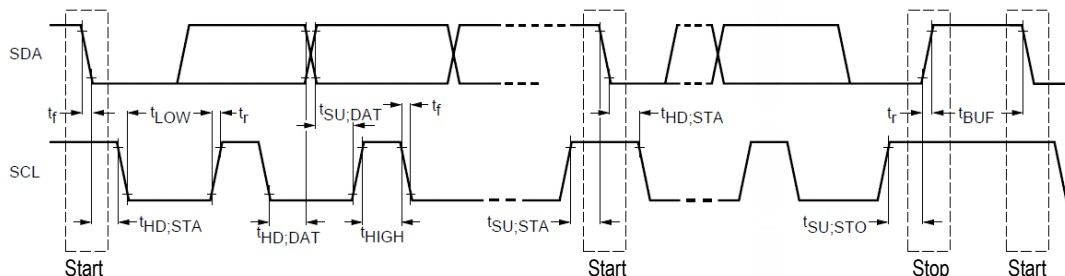
Figure 23 - I 2 C Slave/Synchronous Slave Control Interface Timing Diagram
