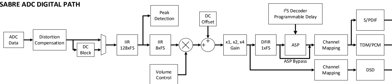
SABRE ADC DIGITAL PATH
