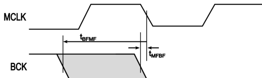
Figure 21 - 45/49MHz MCLK with BCK Phase Relationship
