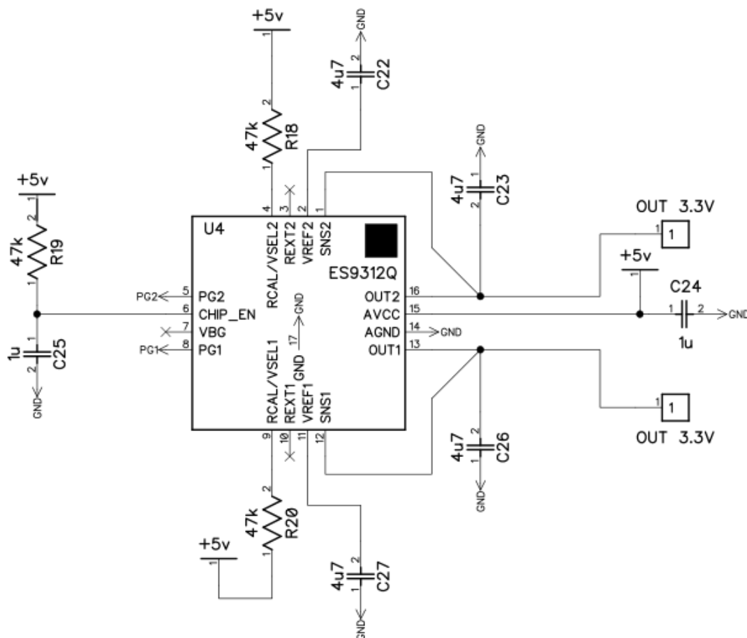
Figure 28 - ES9312Q Reference Voltage Regulator Schematic
