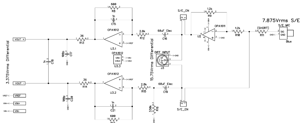
Figure 27 - Reference Schematic ADC Input Stage for Single Ended (S/E) and Differential Input
