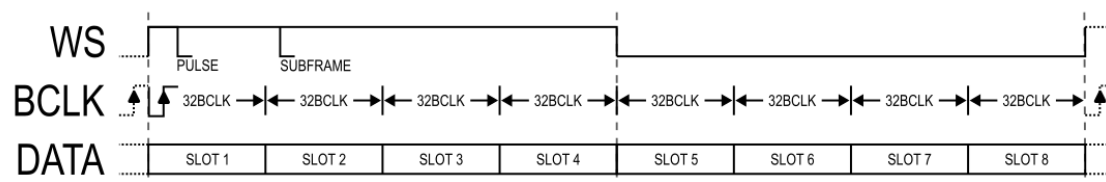
Figure 9 - TDM8 Mode
