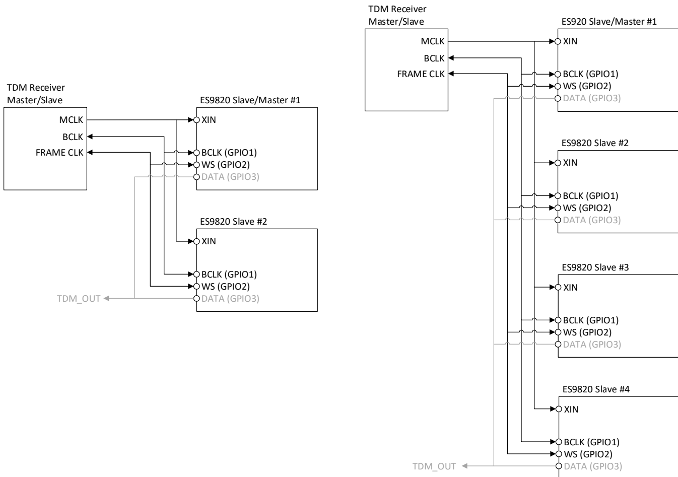
Figure 15 - Connection for Parallel TDM / PCM
