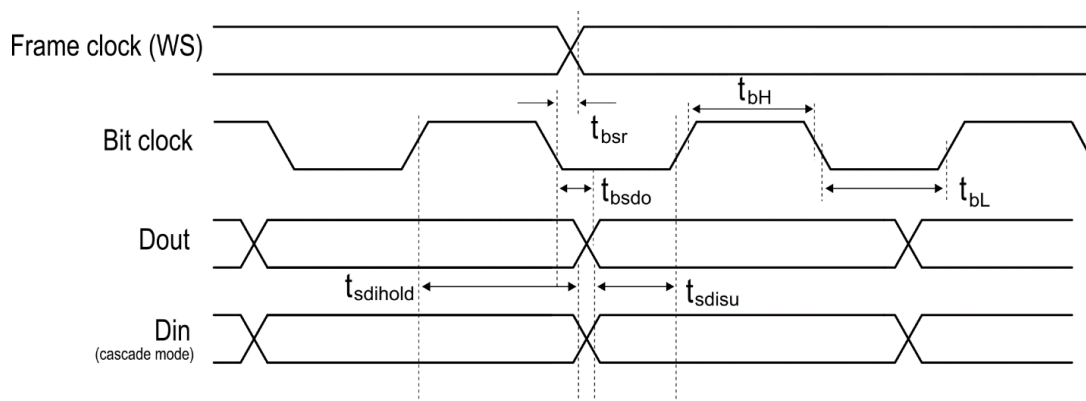
Figure 20 - Audio Interface Timing Requirements
