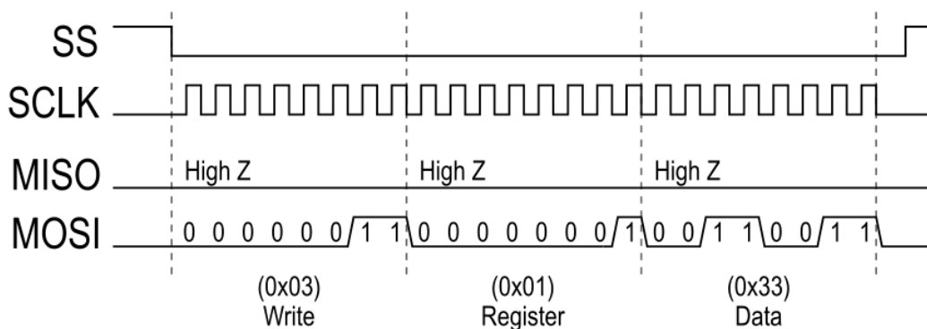
Figure 5 - SPI Single Byte Write
