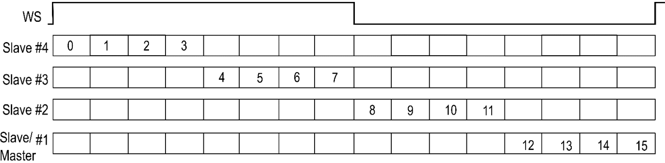
Figure 16 - Channel Mapping and Data Line Composition for TDM in Parallel Mode
