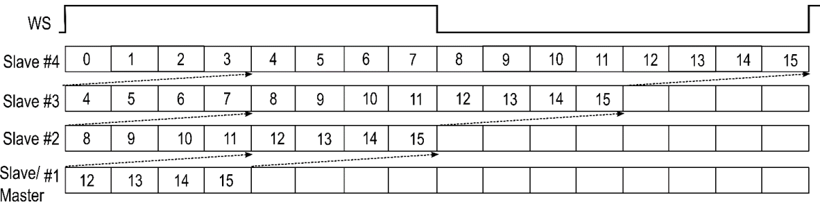
Figure 14 - Channel Cascading and Data Line Composition in TDM Cascade Mode
