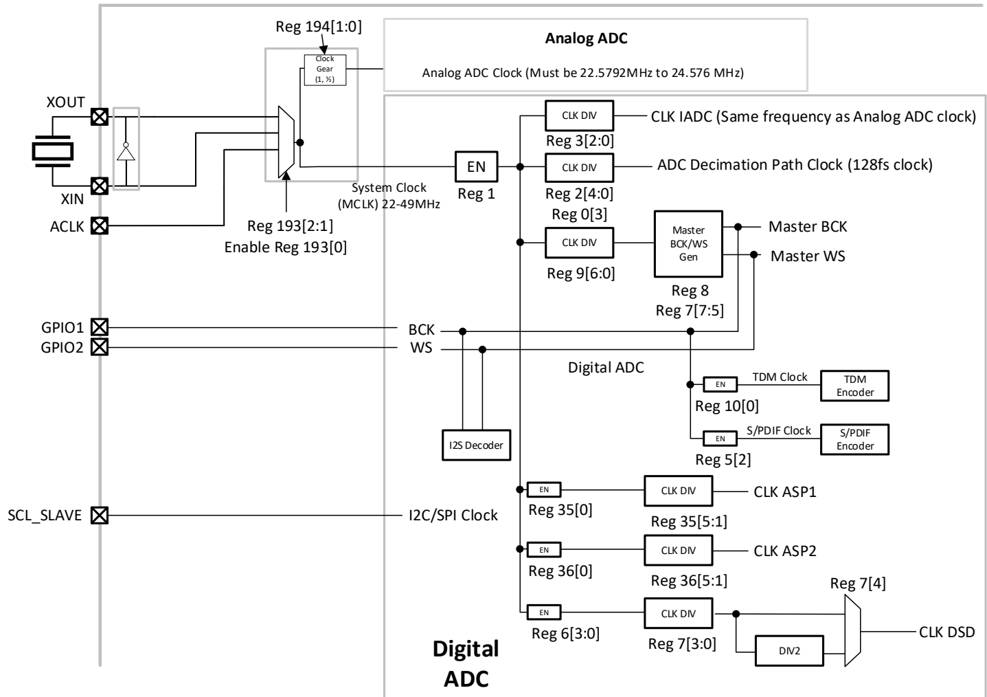
Figure 19 - ES9820 Clock Distribution
