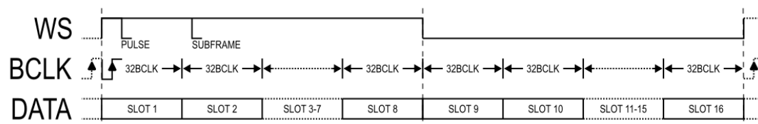
Figure 10 - TDM16 Mode
