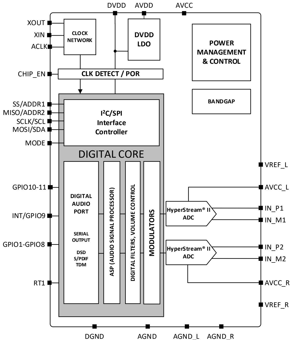
Figure 1 - ES9820 Block Diagram
