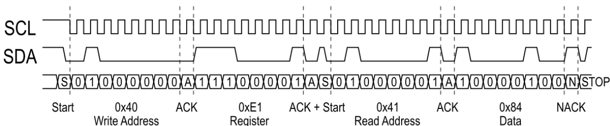
Figure 4 - I 2 C Read Example
