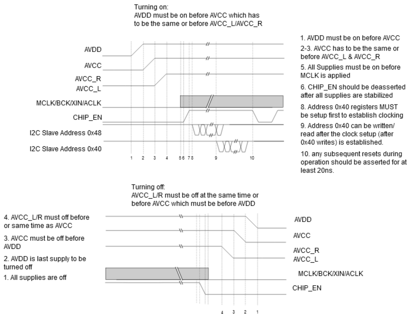
Figure 25 - Recommended Power Up/Down Sequences
