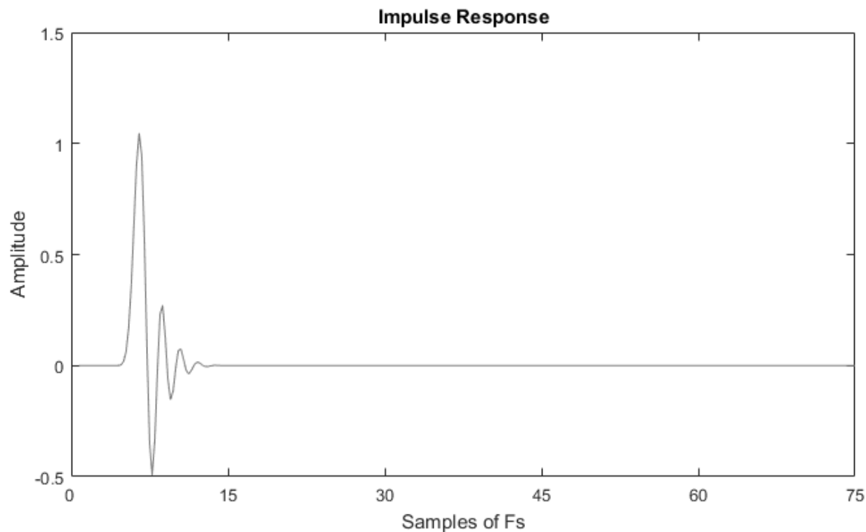
Figure 18 - Minimum Phase 64FS Impulse Response
