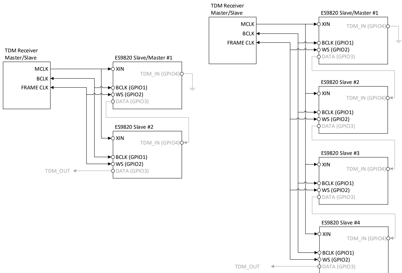
Figure 13 - Connection for TDM Cascade Mode
