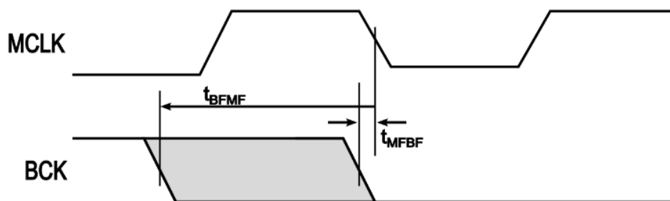
Figure 21 - 45/49MHz MCLK with BCK Phase Relationship
