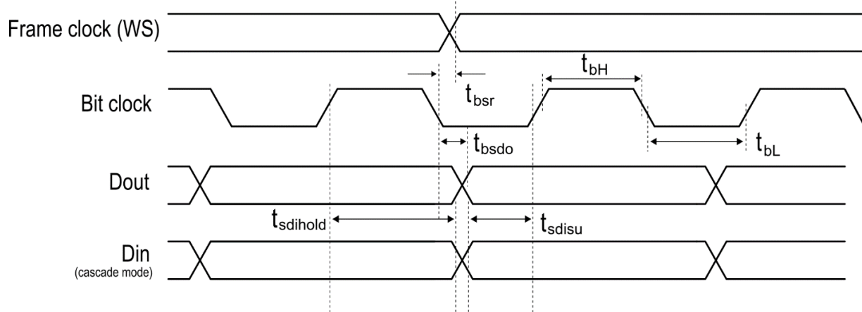
Figure 20 - Audio Interface Timing Requirements
