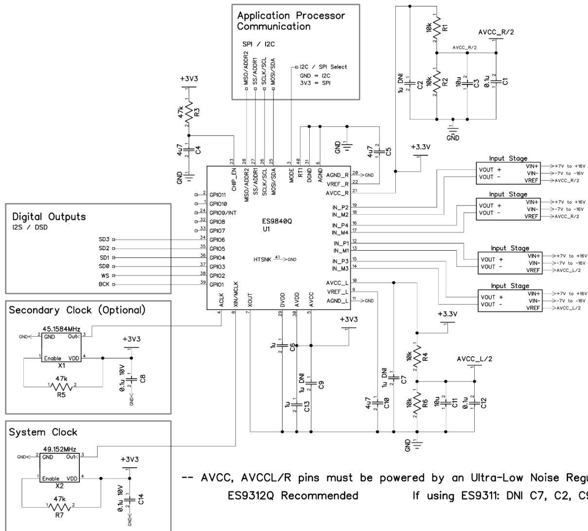
Figure 26 - ES9840Q Reference Schematic for Normal Operation
