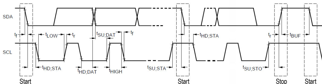
Figure 23 - I 2 C Slave Control Interface Timing Diagram
