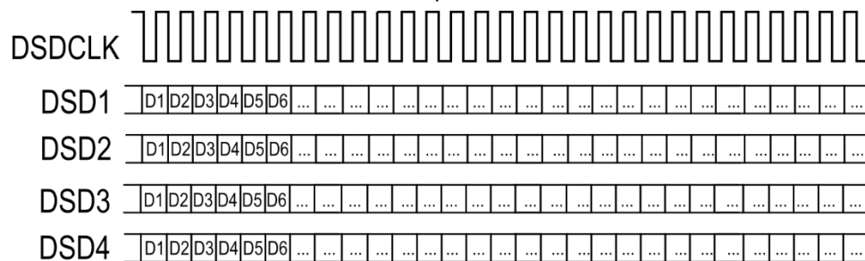
Figure 11 - 4CH DSD Format
