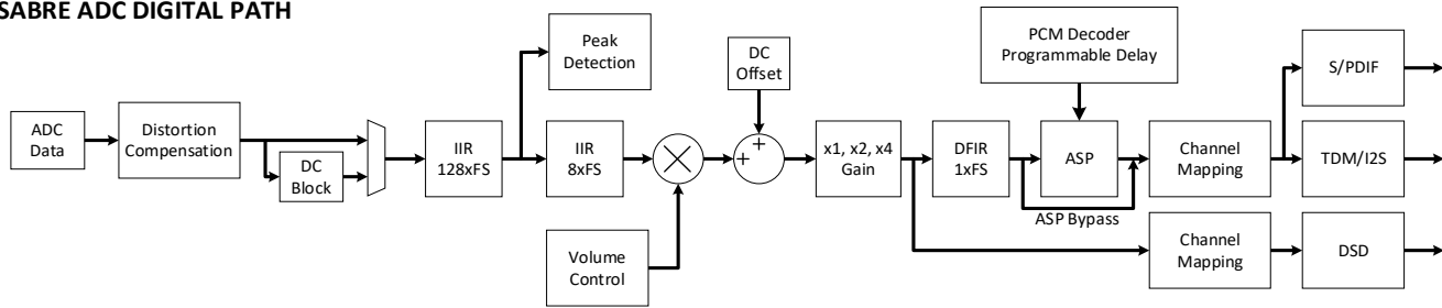
SABRE ADC DIGITAL PATH
