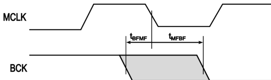
Figure 22 - 22/24MHz MCLK with BCK Phase Relationship
