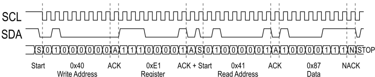
Figure 4 - I 2 C Read Example
