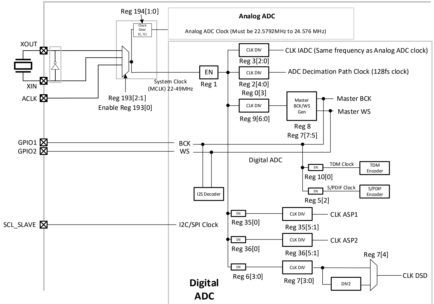
Figure 19 - ES9840 Clock Distribution
