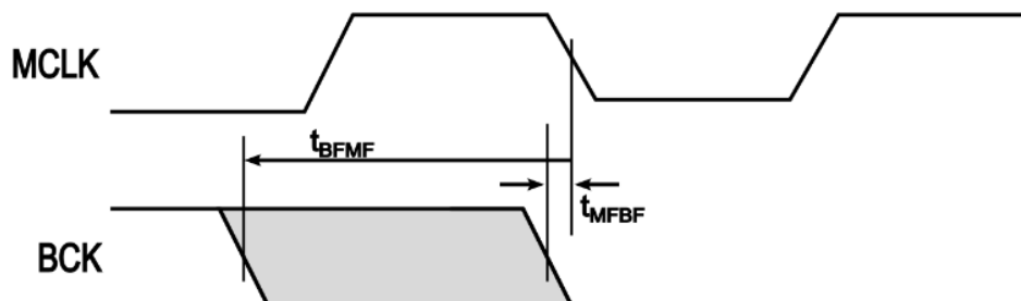
Figure 23 - 45/49MHz MCLK with BCK Phase Relationship
