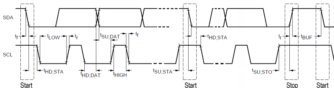
Figure 25 - I 2 C Slave Control Interface Timing Diagram
