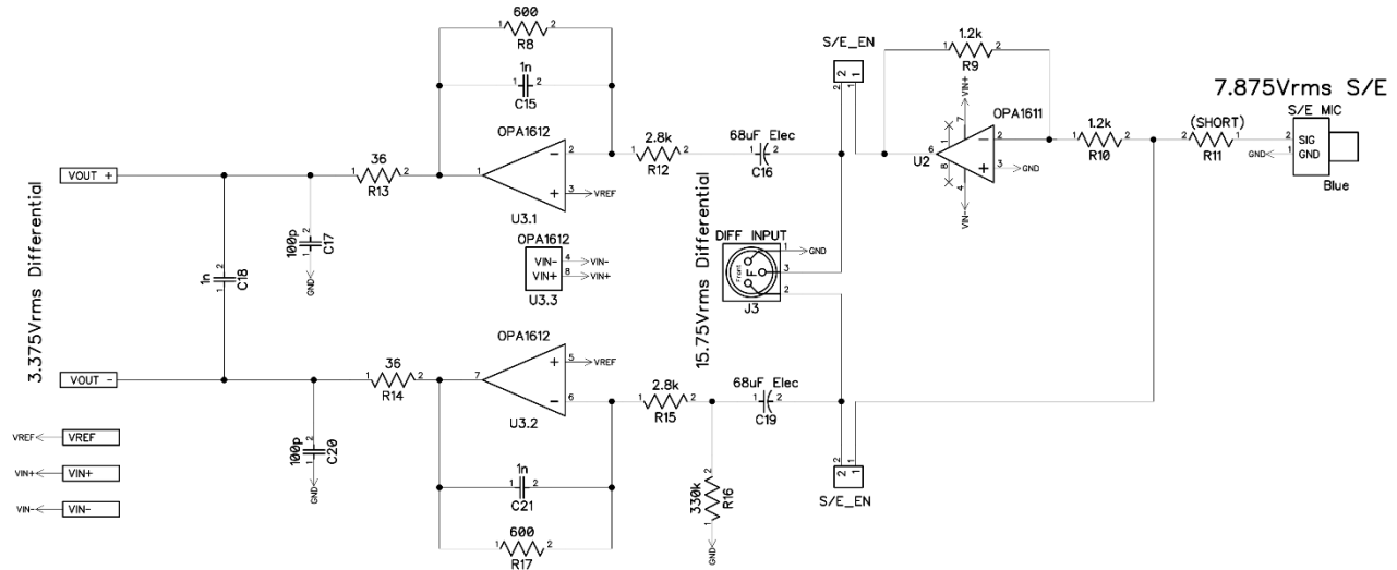
Figure 29 - Reference Schematic ADC Input Stage for Single Ended (S/E) and Differential Input
