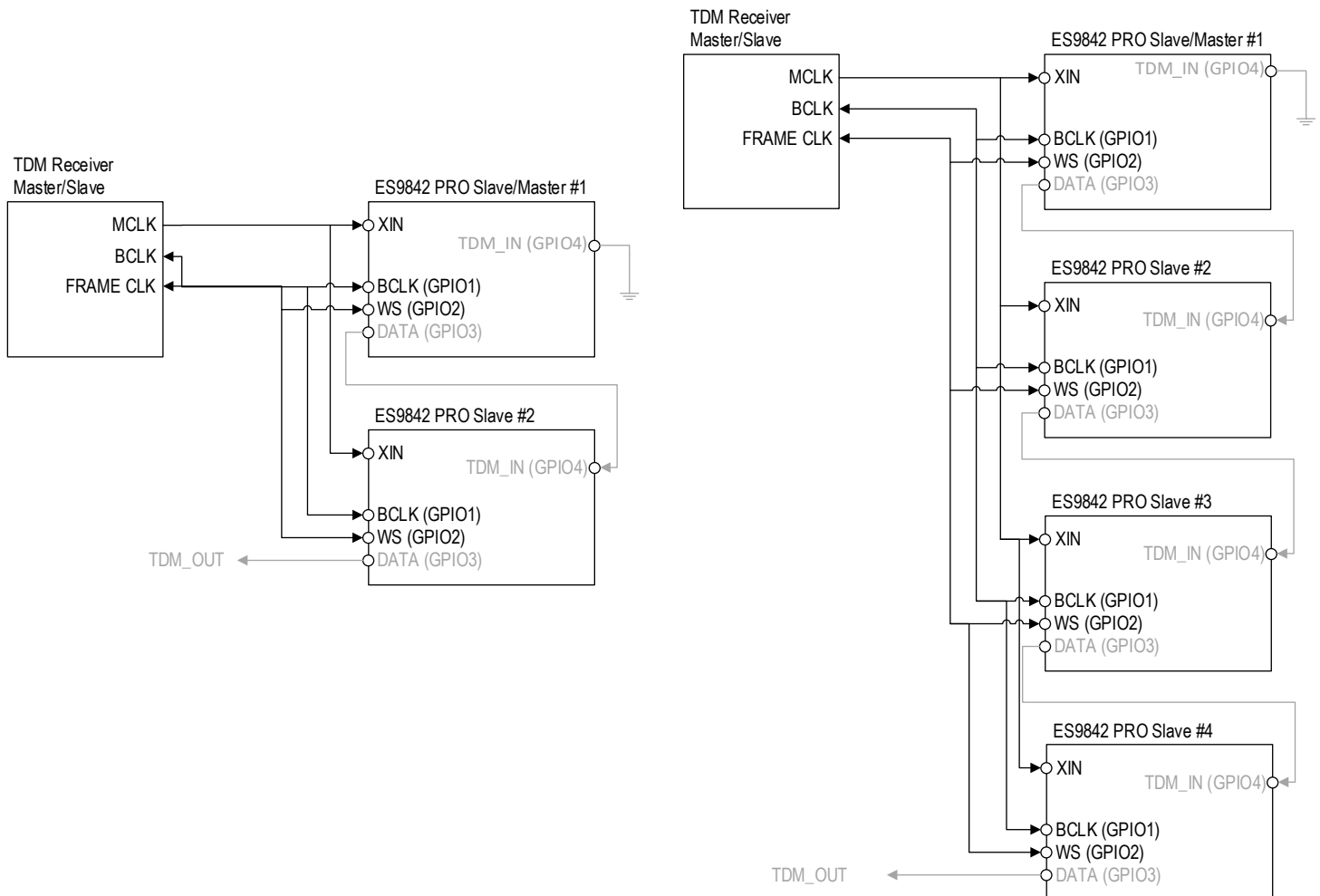
Figure 15 - Connection for TDM Cascade Mode
