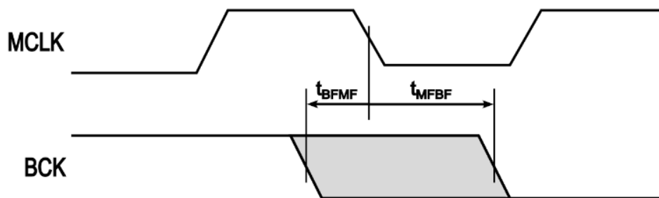
Figure 24 - 22/25MHz MCLK with BCK Phase Relationship
