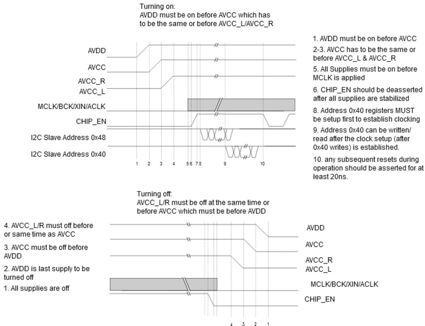
Figure 27 - Recommended Power Up/Down Sequences
