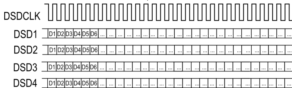
Figure 11 - 2CH DSD Format
