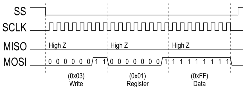
Figure 5 - SPI Single Byte Write
