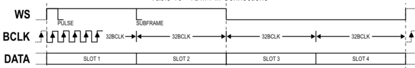
Figure 8 - TDM4 Mode
