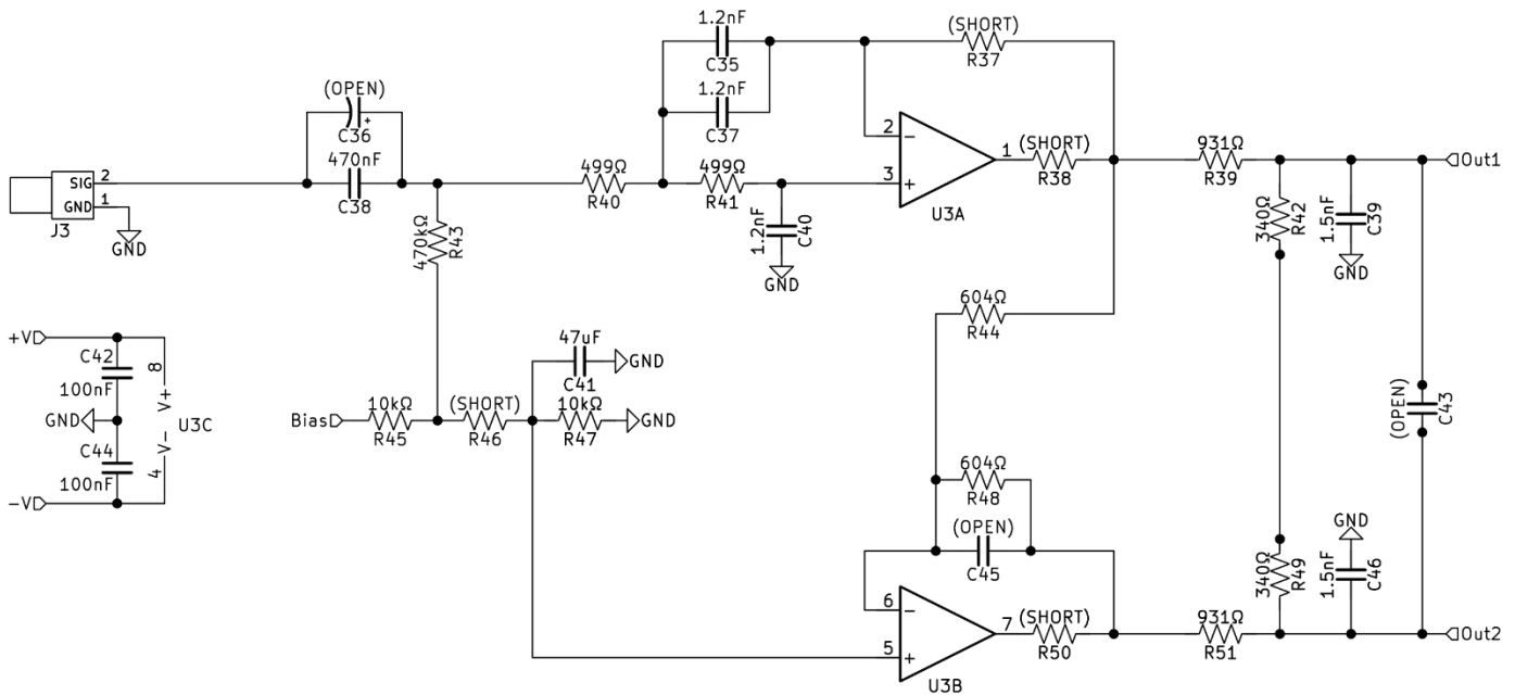
Figure 31 - Recommended Single-Ended Input Stage
