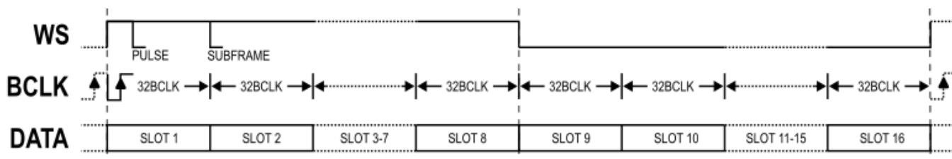
Figure 10 - TDM16 Mode
