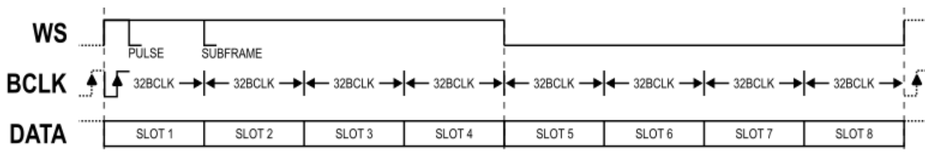
Figure 9 - TDM8 Mode
