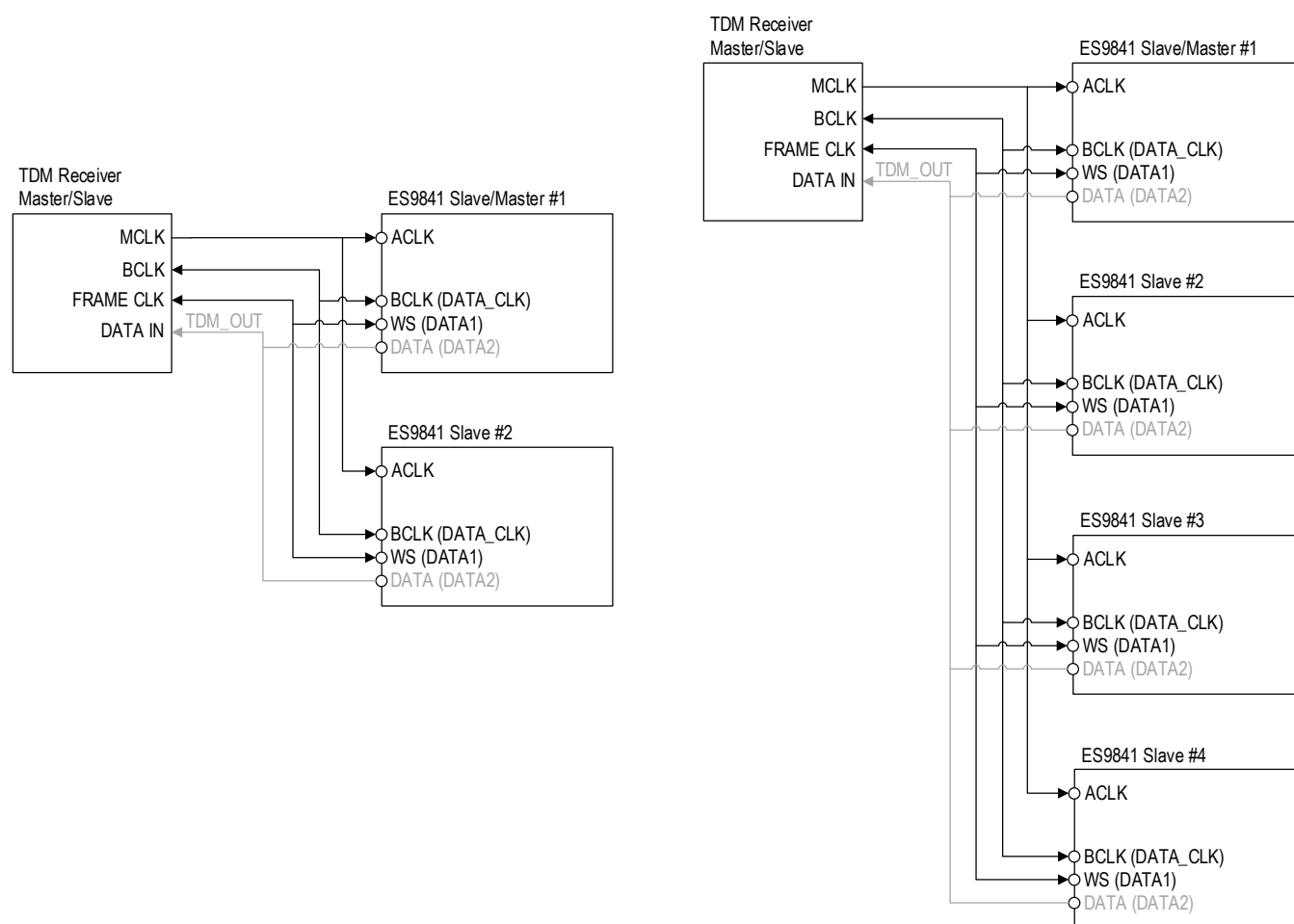
Figure 19 - Example Connection for TDM/PCM Parallel Mode
