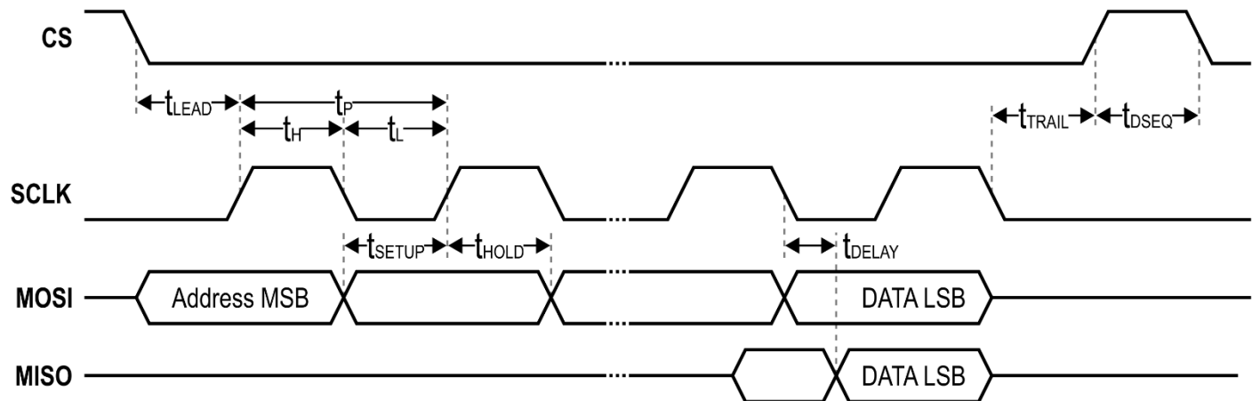
Figure 26 - SPI Slave Interface Timing
