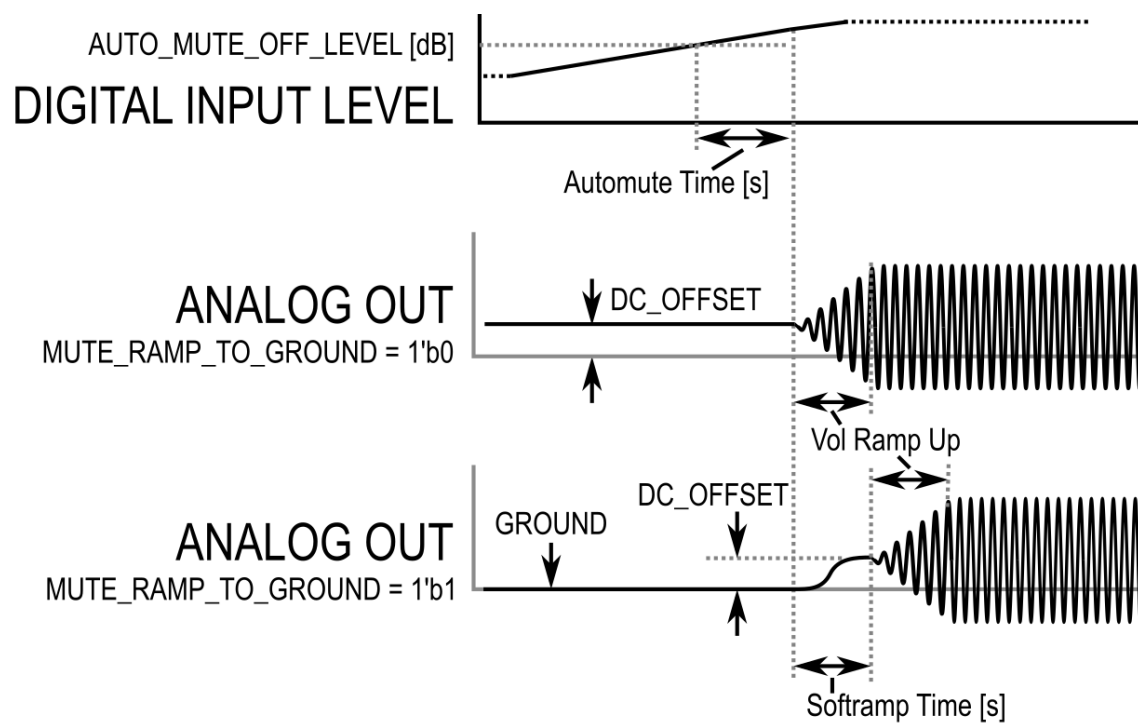
Figure 23 - Automute Disengaging
