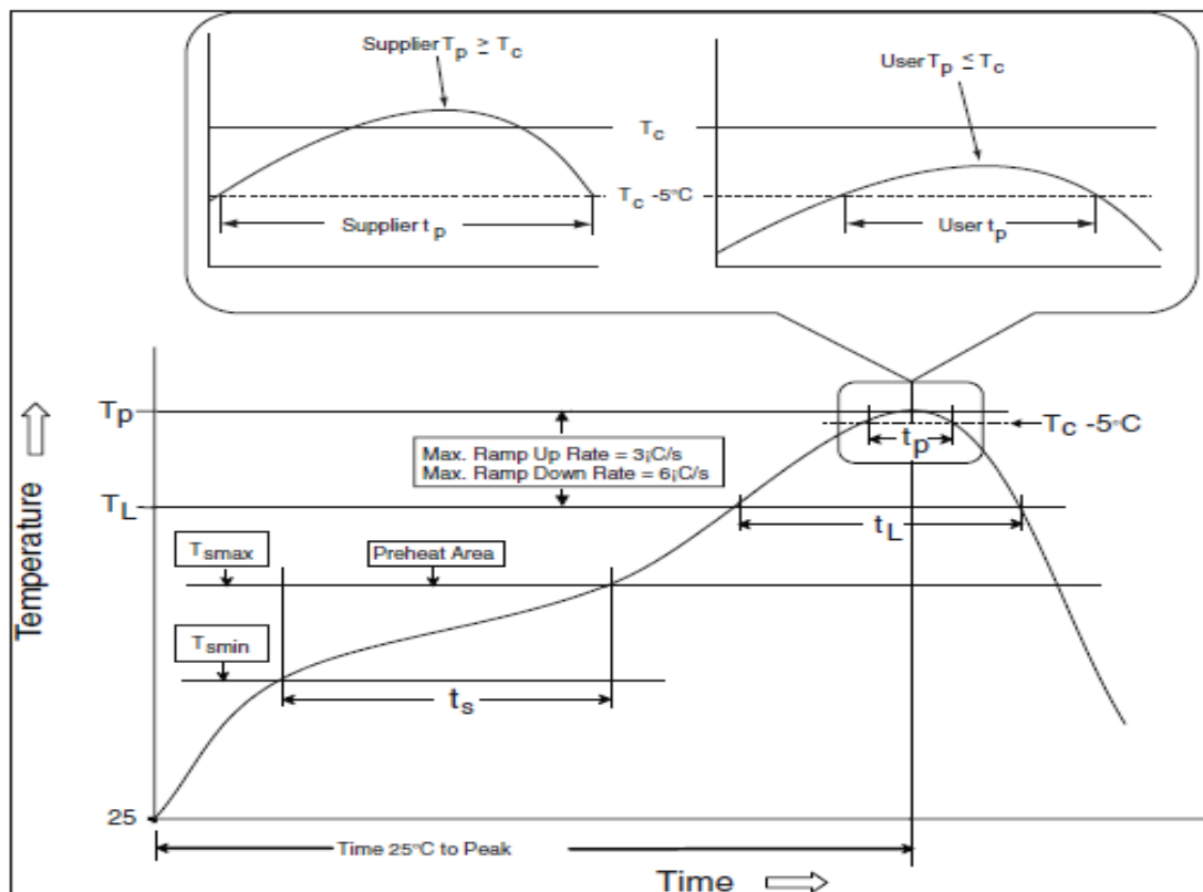
Figure 48 - IR/Convection Reflow Profile (IPC/JEDEC J-STD-020D.1)
