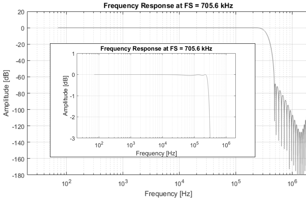
Figure 24 - ADC: Minimum Phase 64FS Frequency Response
