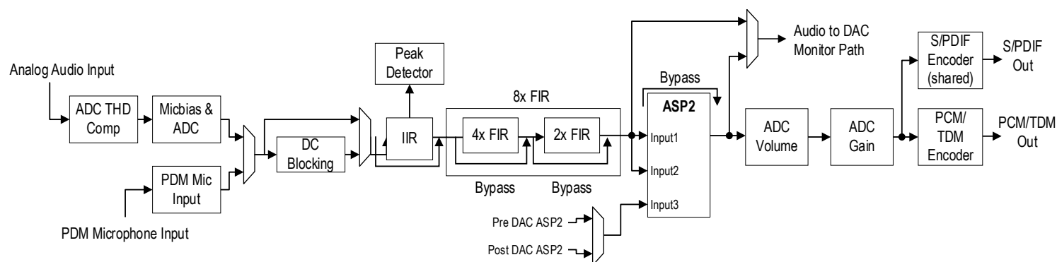
Figure 20 - ADC Digital Signal Path
