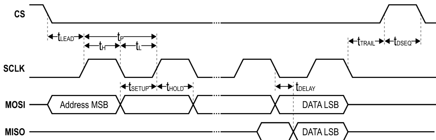
Figure 38 - SPI Slave Interface Timing
