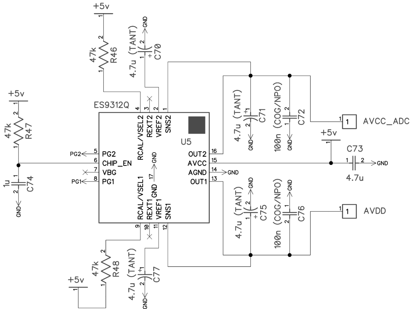
Figure 44 - Recommended Power Supply
