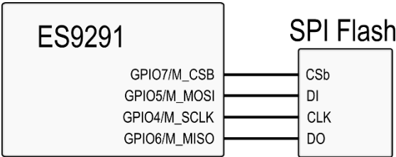
Figure 16 - Example SPI Flash Schematic
