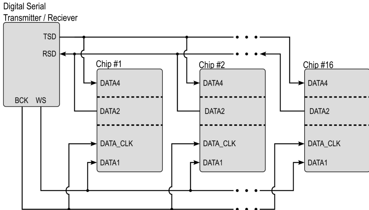
Figure 29 - TDM Parallel Configuration
