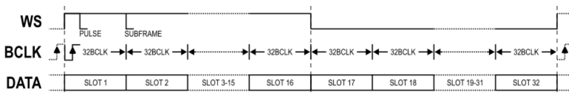
Figure 12 - TDM32 Mode
