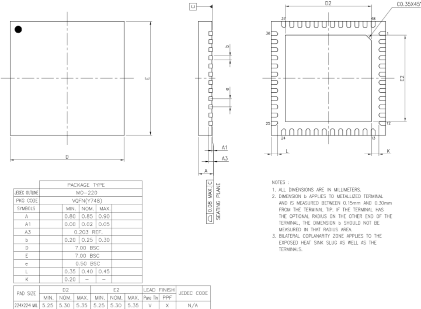
Figure 46 - ES9291 48 QFN Package Dimensions
