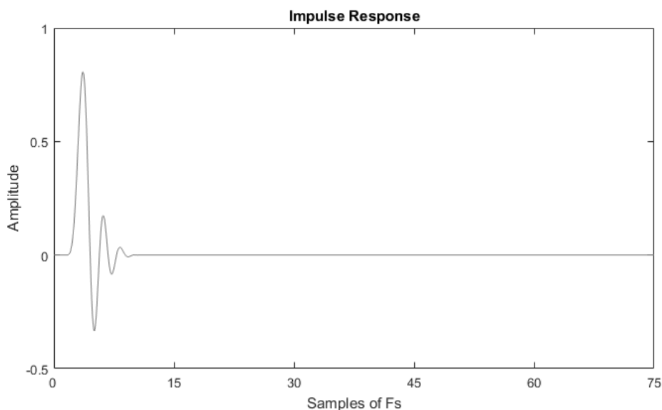
Figure 27 - DAC: Minimum Phase 64FS Impulse Response
