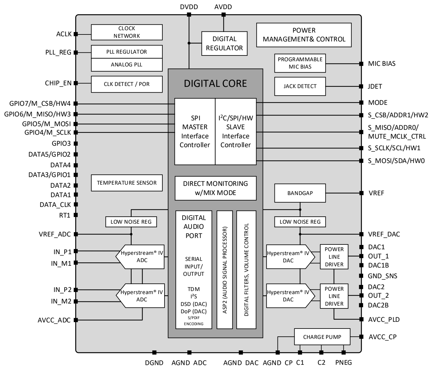
Figure 1 - ES9291 Functional Block Diagram
