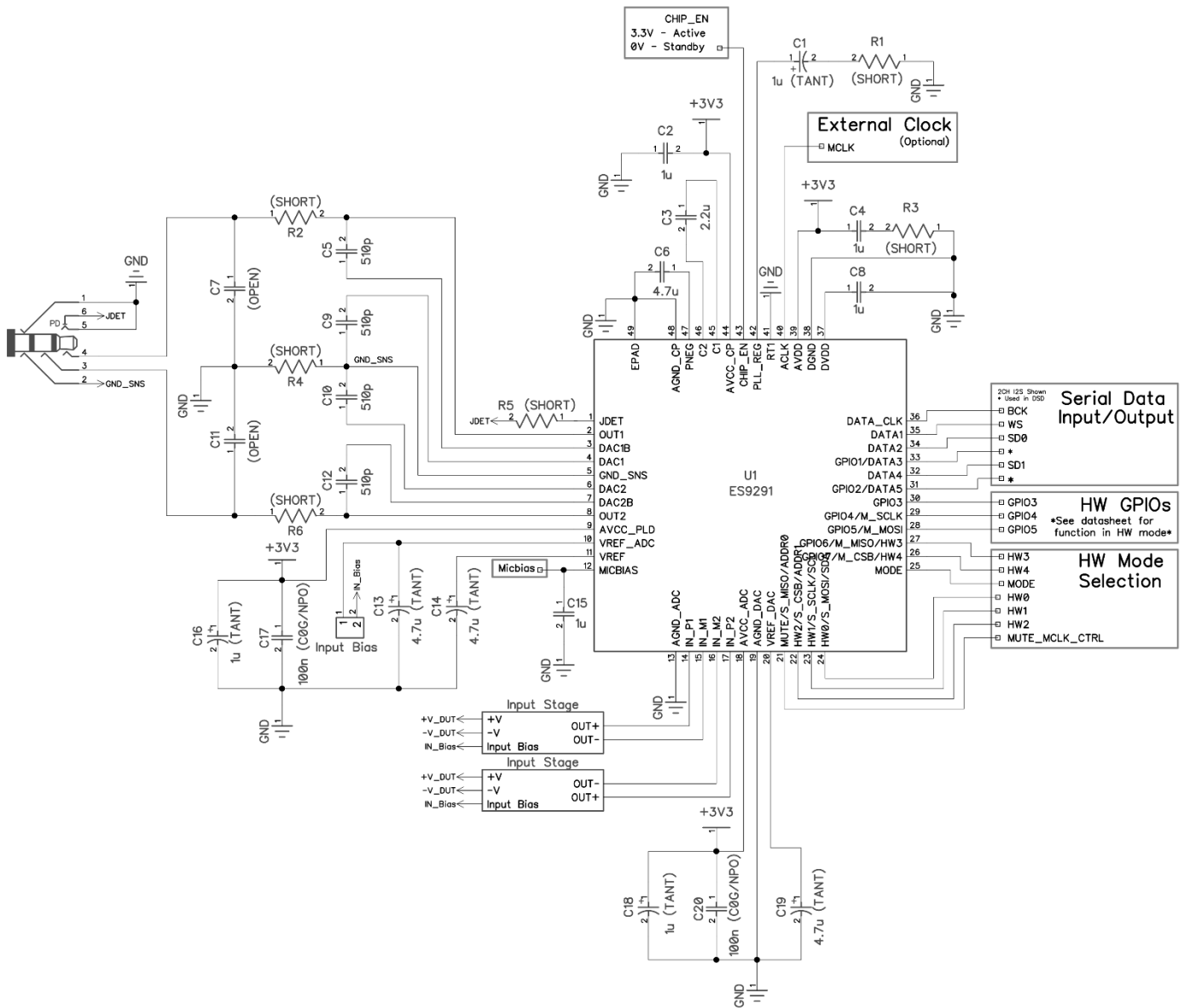
Figure 40 - ES9291 Hardware Mode Reference Schematic
