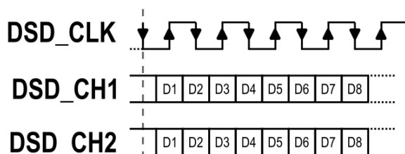
Figure 13 - DSD Format, 1-bit stream
