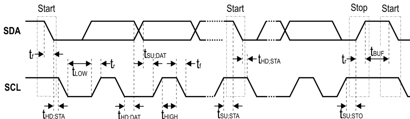
Figure 37 - I 2 C Slave Control Interface Timing
