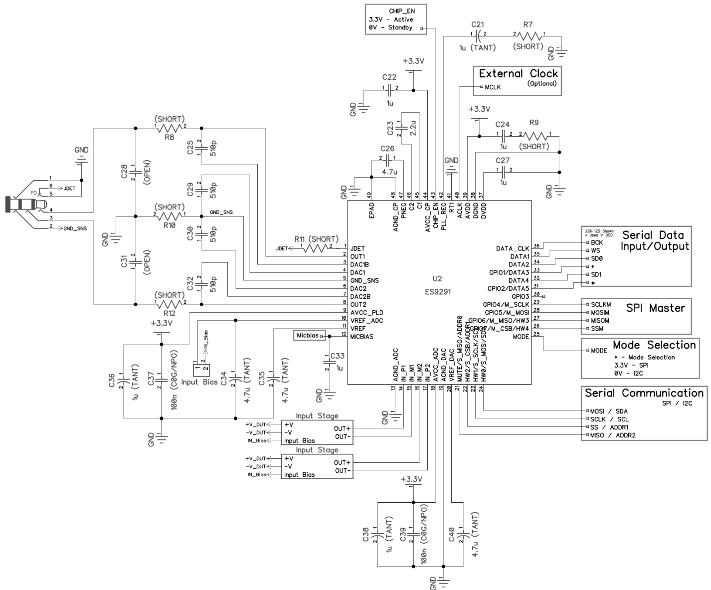
Figure 41 - ES9291 Software Mode Reference Schematic
