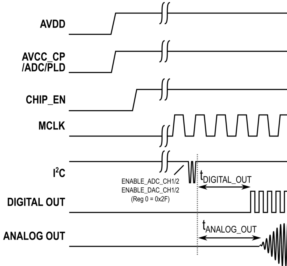
Figure 39 - Recommended Power Up Sequence
