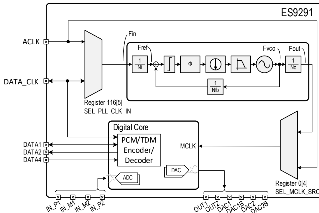
Figure 31 - Functional Block Diagram of ES9291 APLL
