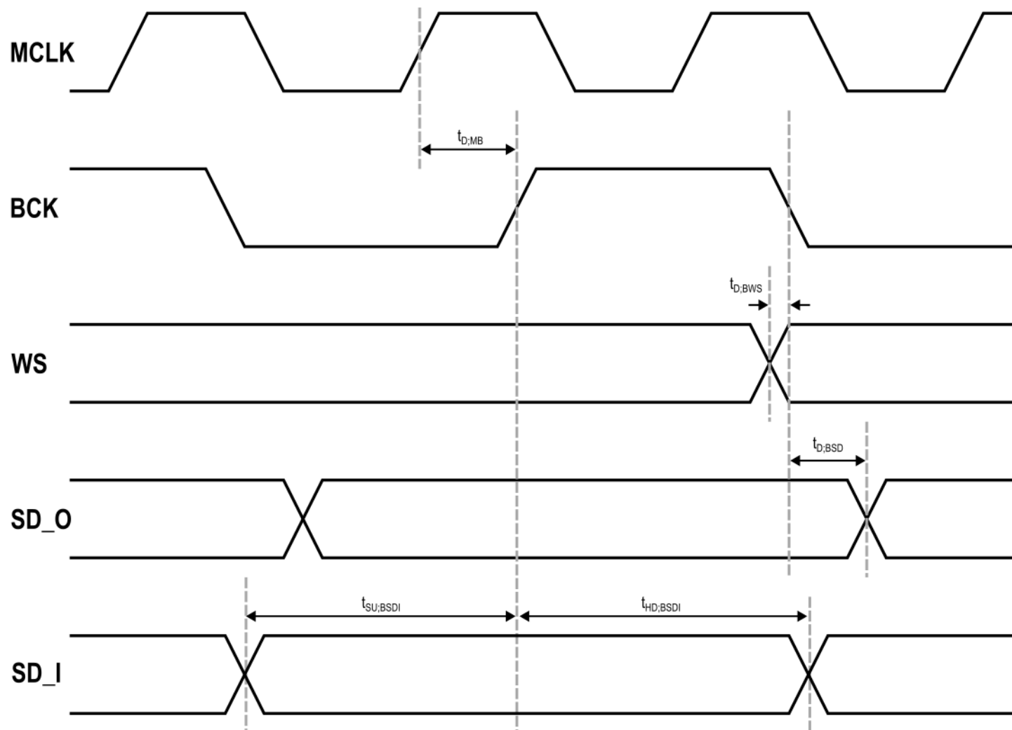
Figure 35 - Master Mode TDM Timing Diagram
