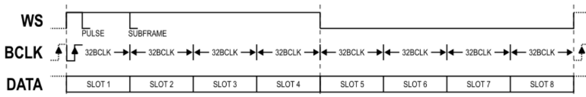
Figure 10 - TDM8 Mode
