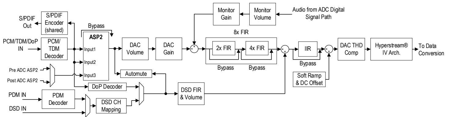
Figure 21 - DAC Digital Signal Path
