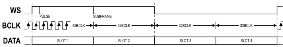
Figure 9 - TDM4 Mode
