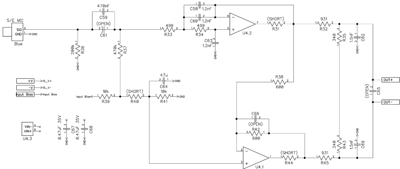
Figure 43 - Single-Ended Input Stage Reference Schematic
