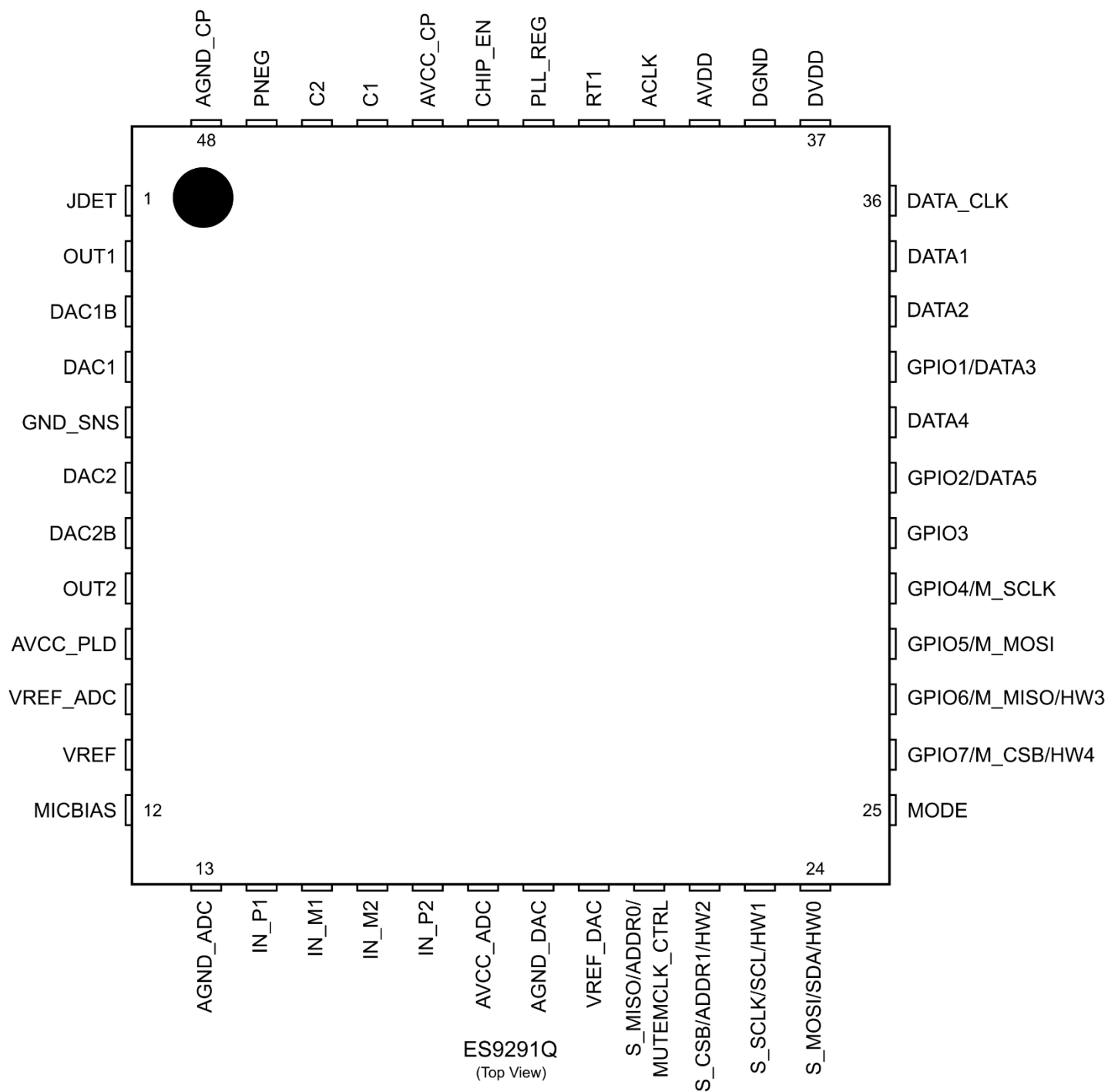
Figure 2 - 48 QFN Pinout
