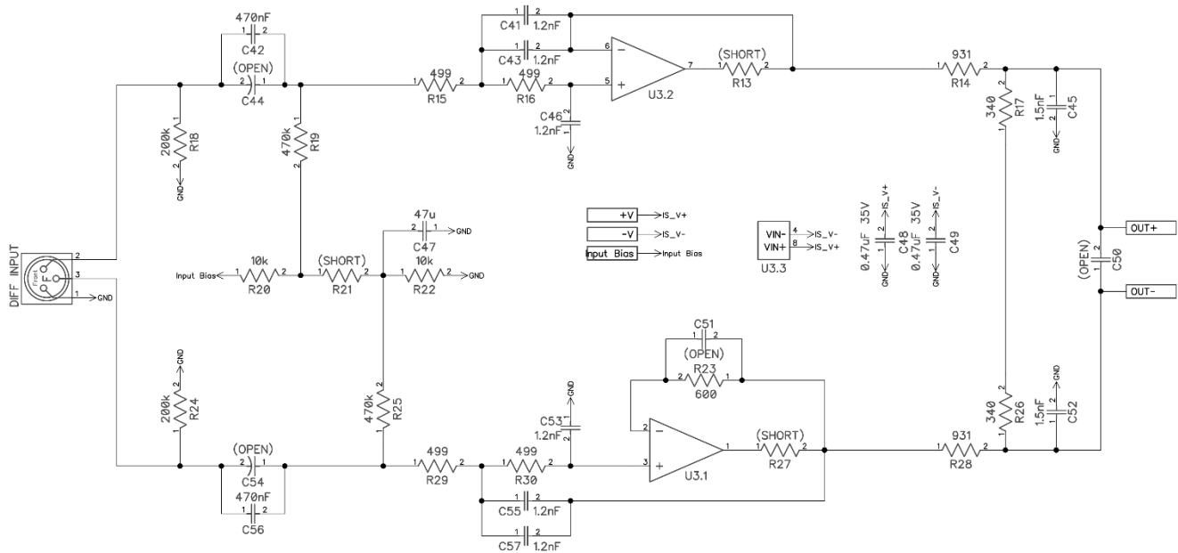
Figure 42 - Differential Input Stage Reference Schematic
