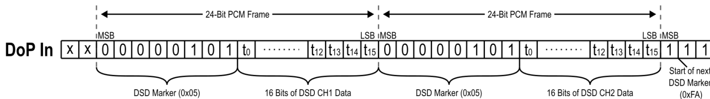
Figure 14 - DoP Format
