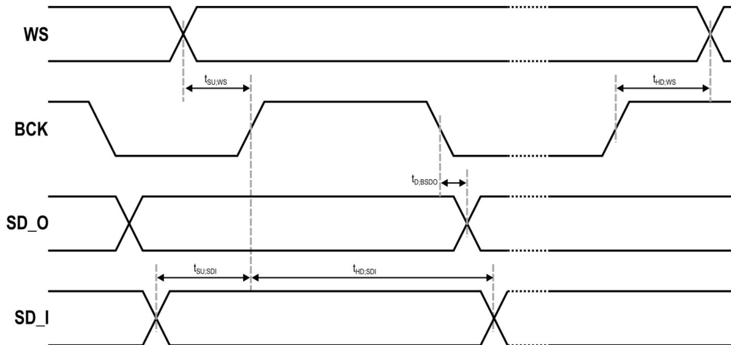
Figure 36 - Slave Mode TDM Timing Diagram
