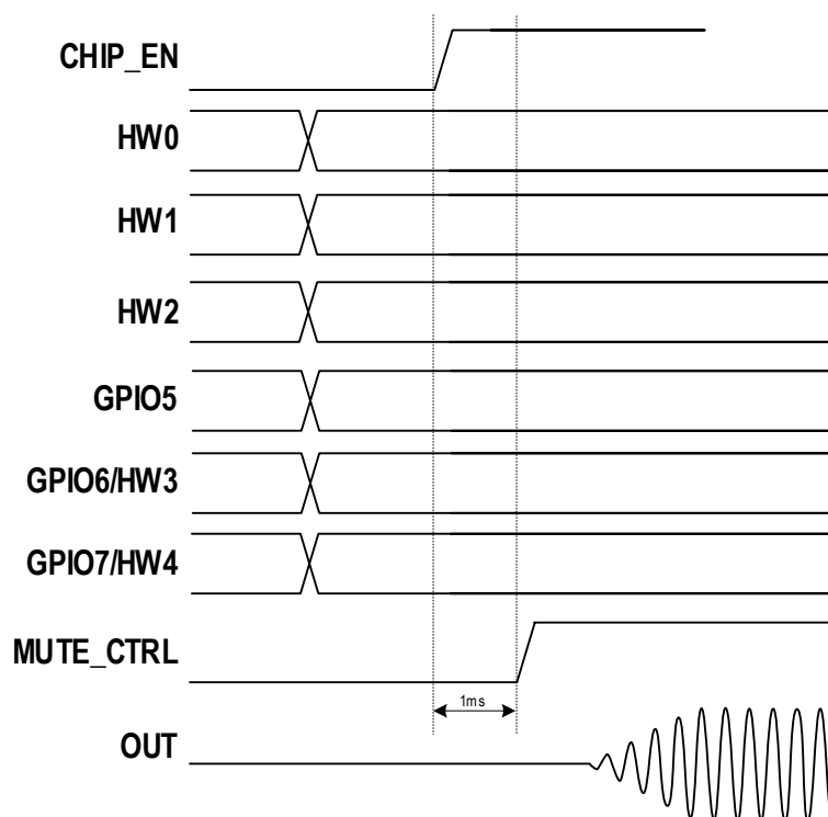
Figure 6 - Hardware Mode Startup Sequence
