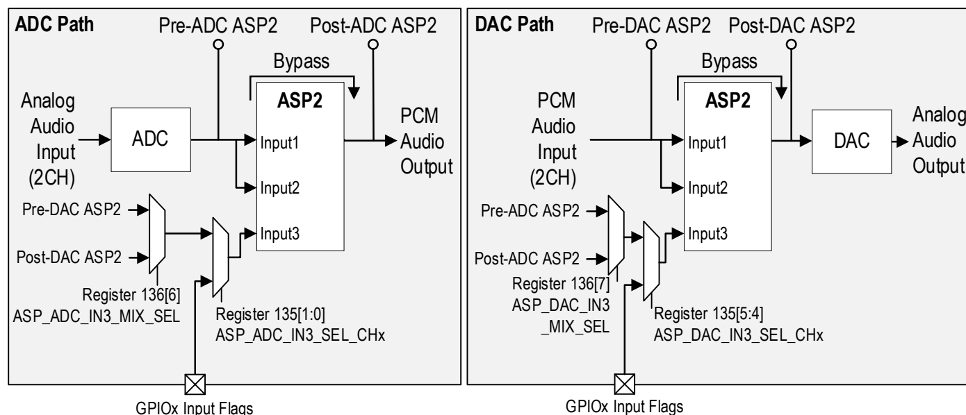
Figure 19 - ES9291 ASP2 Advanced Mixing
