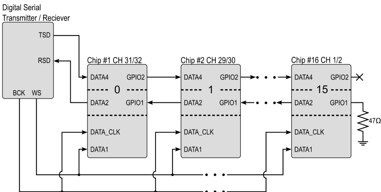
Figure 28 - Daisy Chain Configuration
