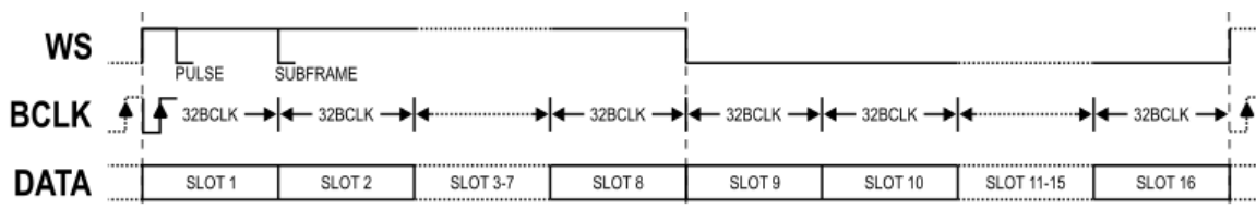
Figure 11 - TDM16 Mode
