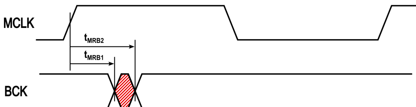
Figure 33 - 45/49M MCLK with BCK Phase Relationship
