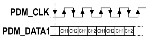
Figure 15 - PDM 2 Channel Format
