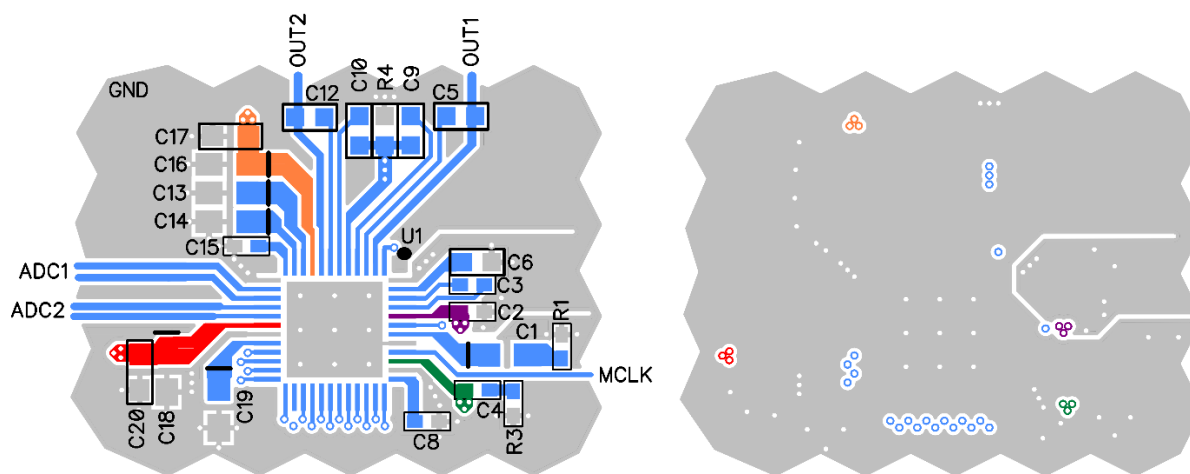
Figure 45 - ES9291 Recommended PCB Layout Guidelines
