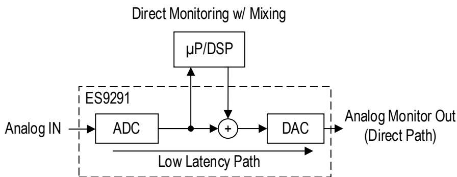
Figure 7 - Direct Monitoring Path
