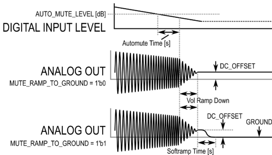
Figure 22 - Automute Engaging
