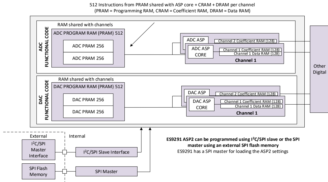
Figure 18 - ASP2 Overview
