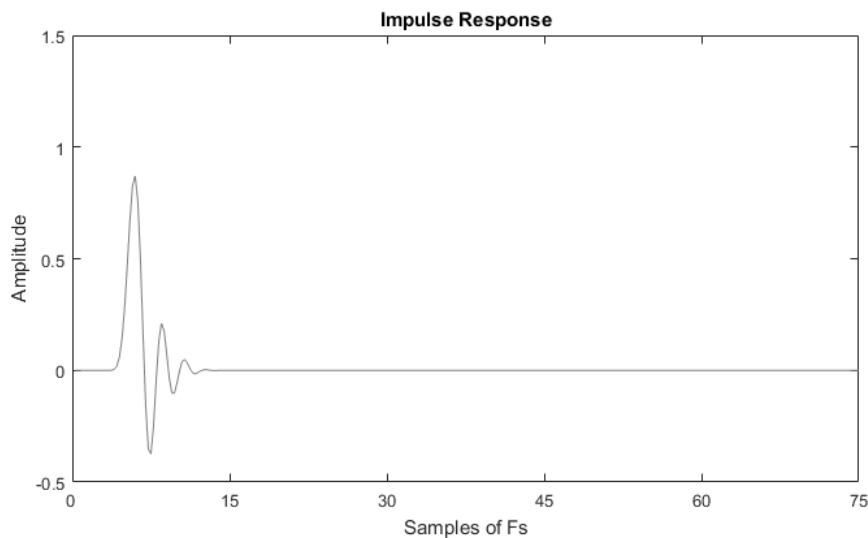
Figure 25 - ADC: Minimum Phase 64FS Impulse Response
