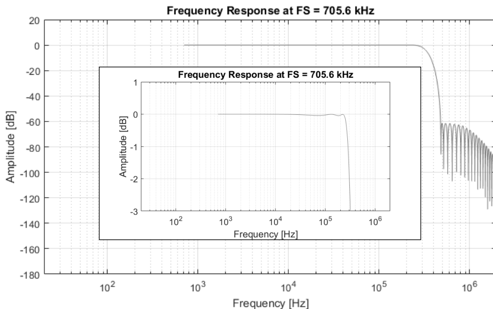
Figure 26 - DAC: Minimum Phase 64FS Frequency Response
