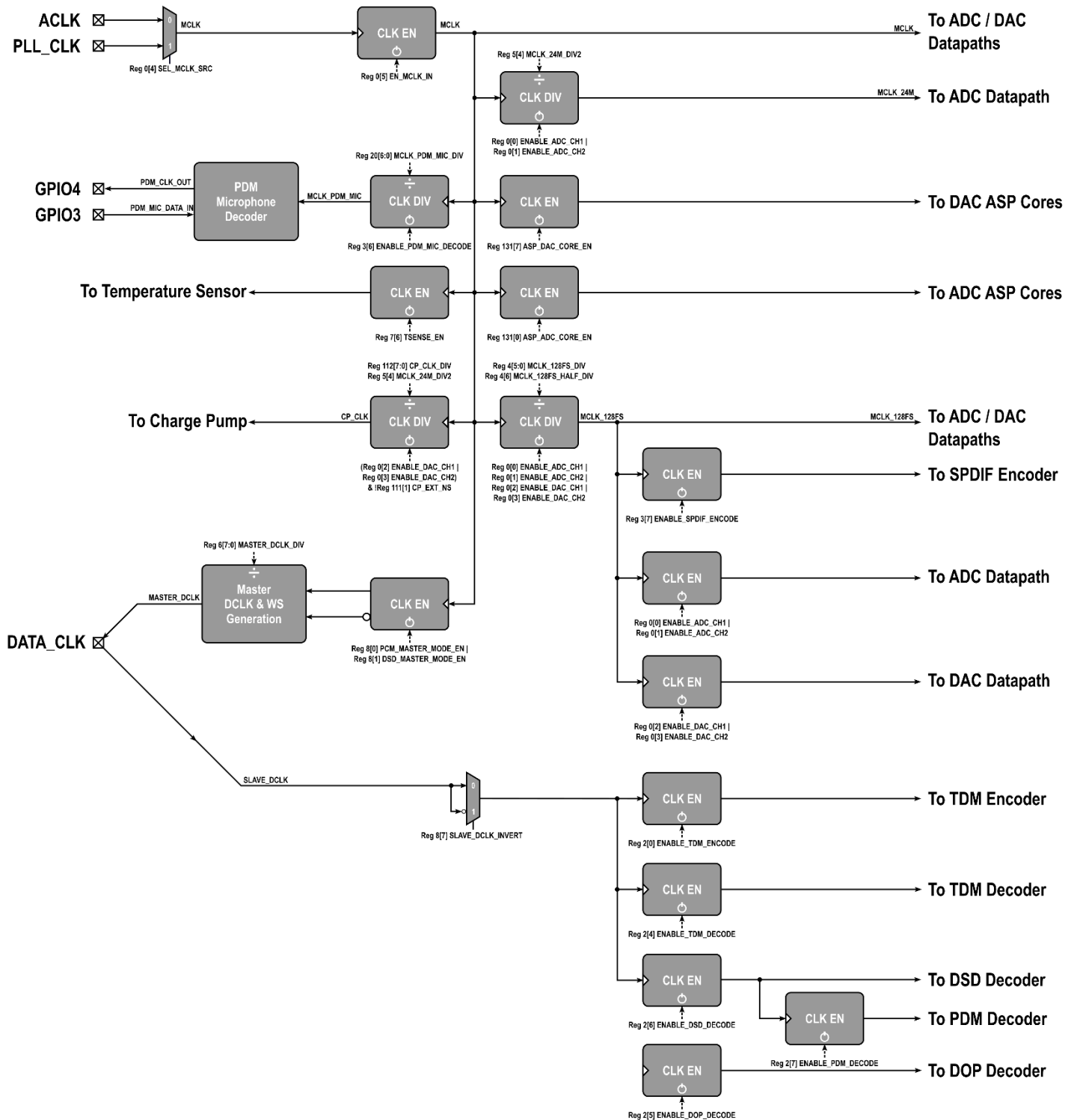
Figure 30 - Clock Distribution
